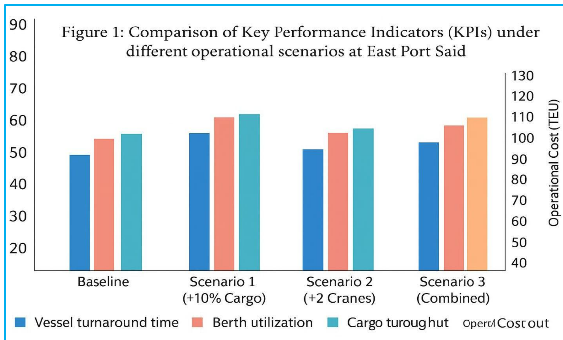
Figure (1) Comparison of Key Performance Indicators (KPIs) Under Different Operational Scenarios at East Port Said.
