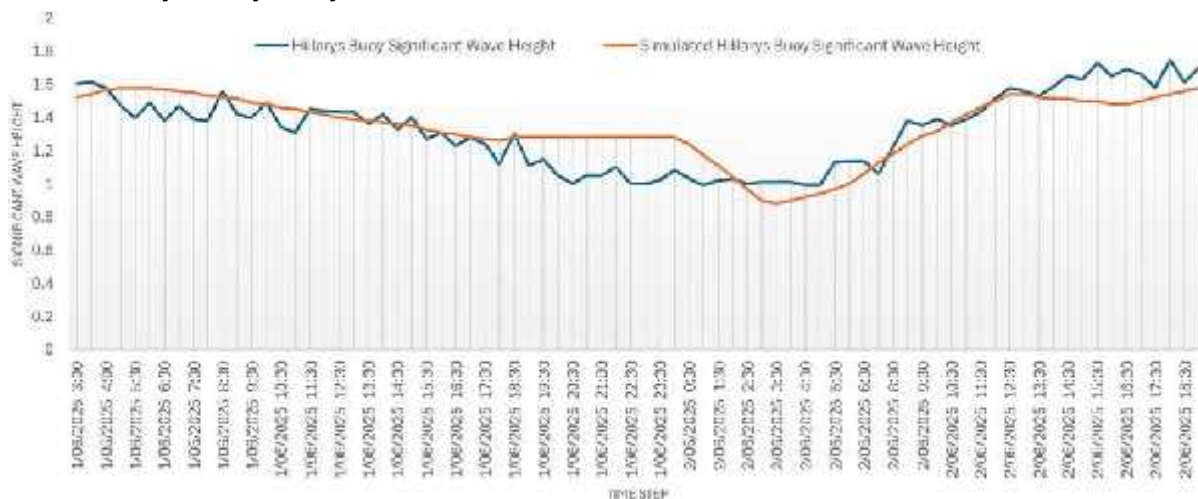
Figure 17: Simulated H_s and the recorded H_s by Hillarys buoy, located at Lat - 31.852°, Long 115.647° WGS 84
