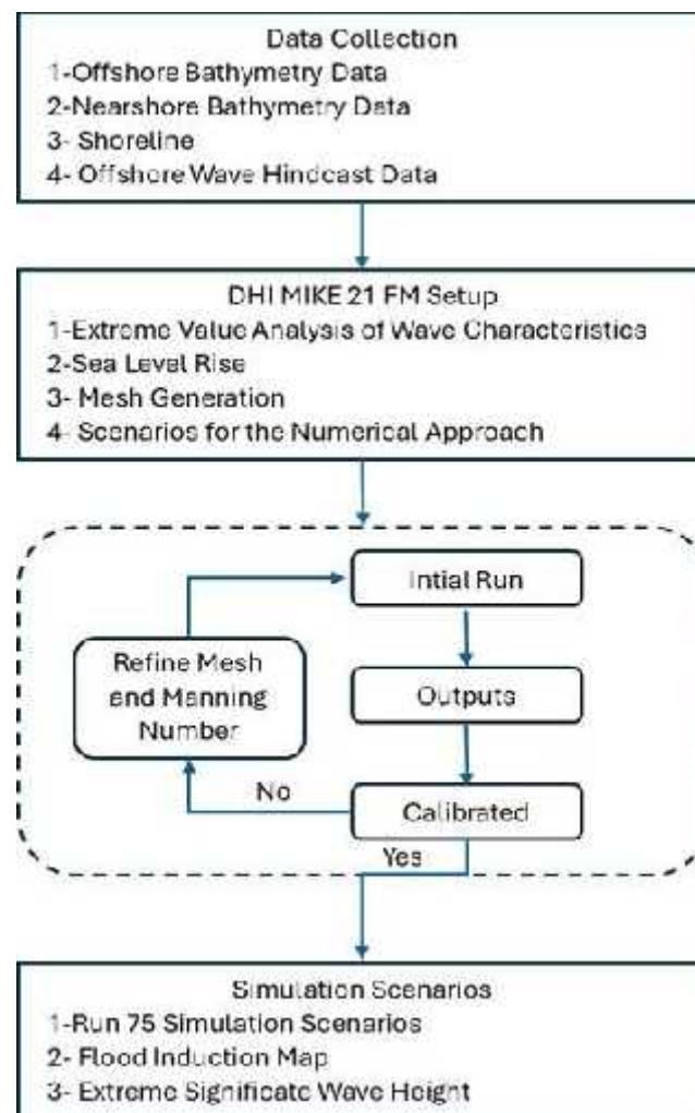
Figure 2: Numerical Methodology Flow Chart followed for the Study.
