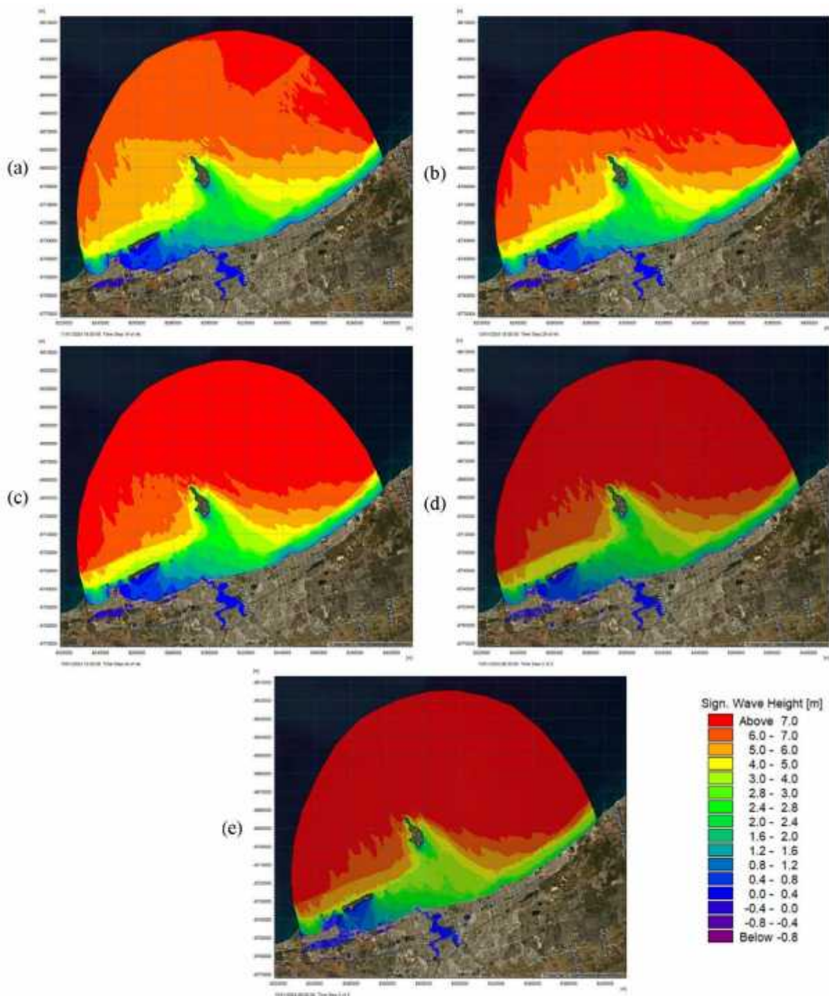
Figure 20: Highest Wave Amplitude of direction 270° with SLR RCP / SSP 8.5 LC for Perth (a) H_s for 1-year R.P, (b) H_s for 5-year R.P, (c) H_s for 20-year R.P, (d) H_s for 50-year R.P, (e) H_s for 100-year R.P.
