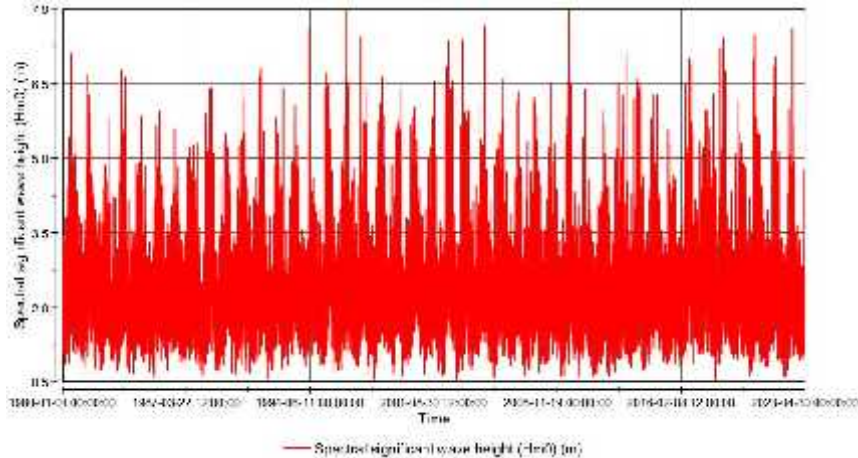
Figure 5: Wave Dataset (1) Spectral H_s , from 1980 till 2023, for the Offshore Wave of Perth, WA
