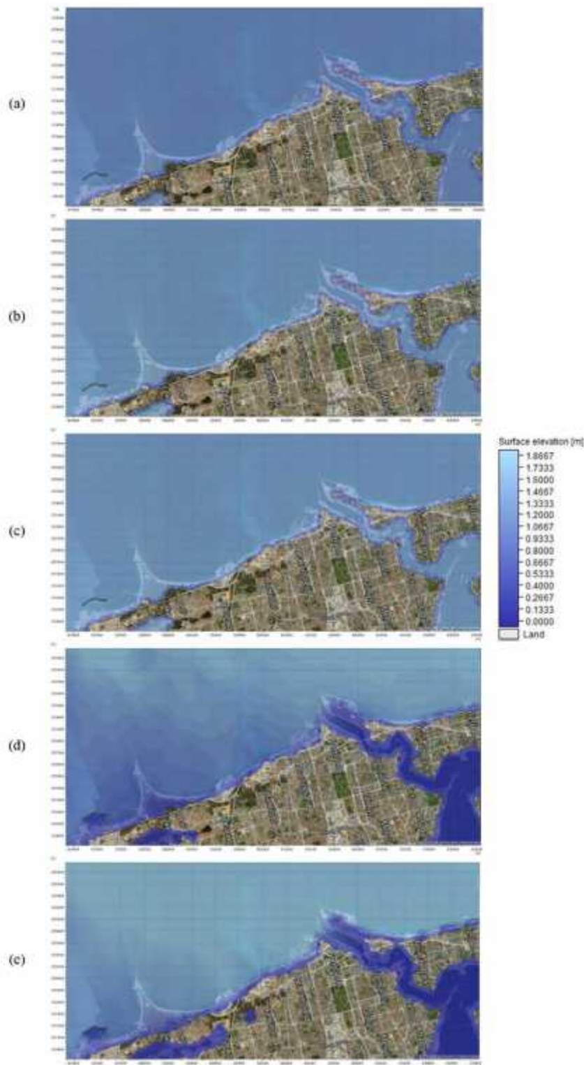
Figure 21: Flooded Footprint due to extreme Wave Events blowing from direction 270° with SLR RCP / SSP 8.5 LC for Fremantle, Perth (a) H_s for 1-year R.P, (b) H_s for 5-year R.P, (c) H_s for 20-year R.P, (d) H_s for 50-year R.P, (e) H_s for 100-year R.P
