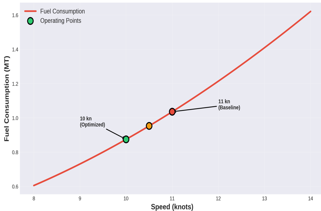
Cubic Relationship: Speed vs Fuel Consumption
