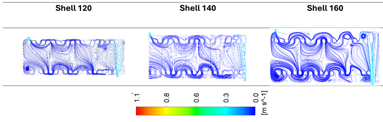
Figure 6 : Streamline for different diameters
