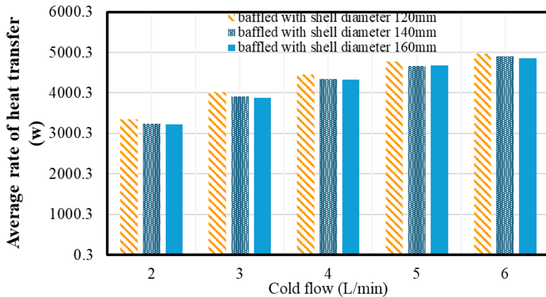
Figure 8 : The rate of heat transfer for different structural arrangements
