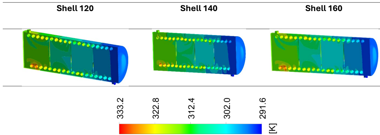
Figure 5 : Temperature contour for different modifications
