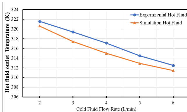
Figure 3 : Comparison between the experimental and numerical hot fluid temperature
