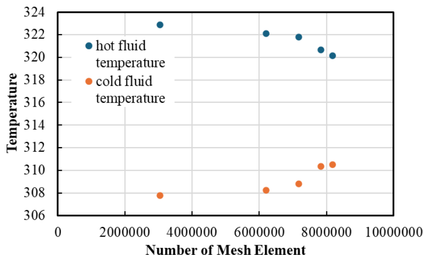
Figure 4 : Mesh Independence Study
