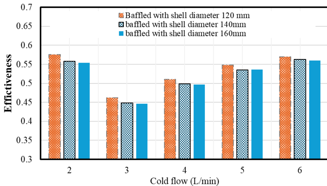
Figure 7 : Effectiveness for different structural arrangements
