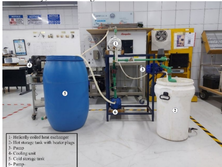
Figure 2 : Experimental Setup layout
