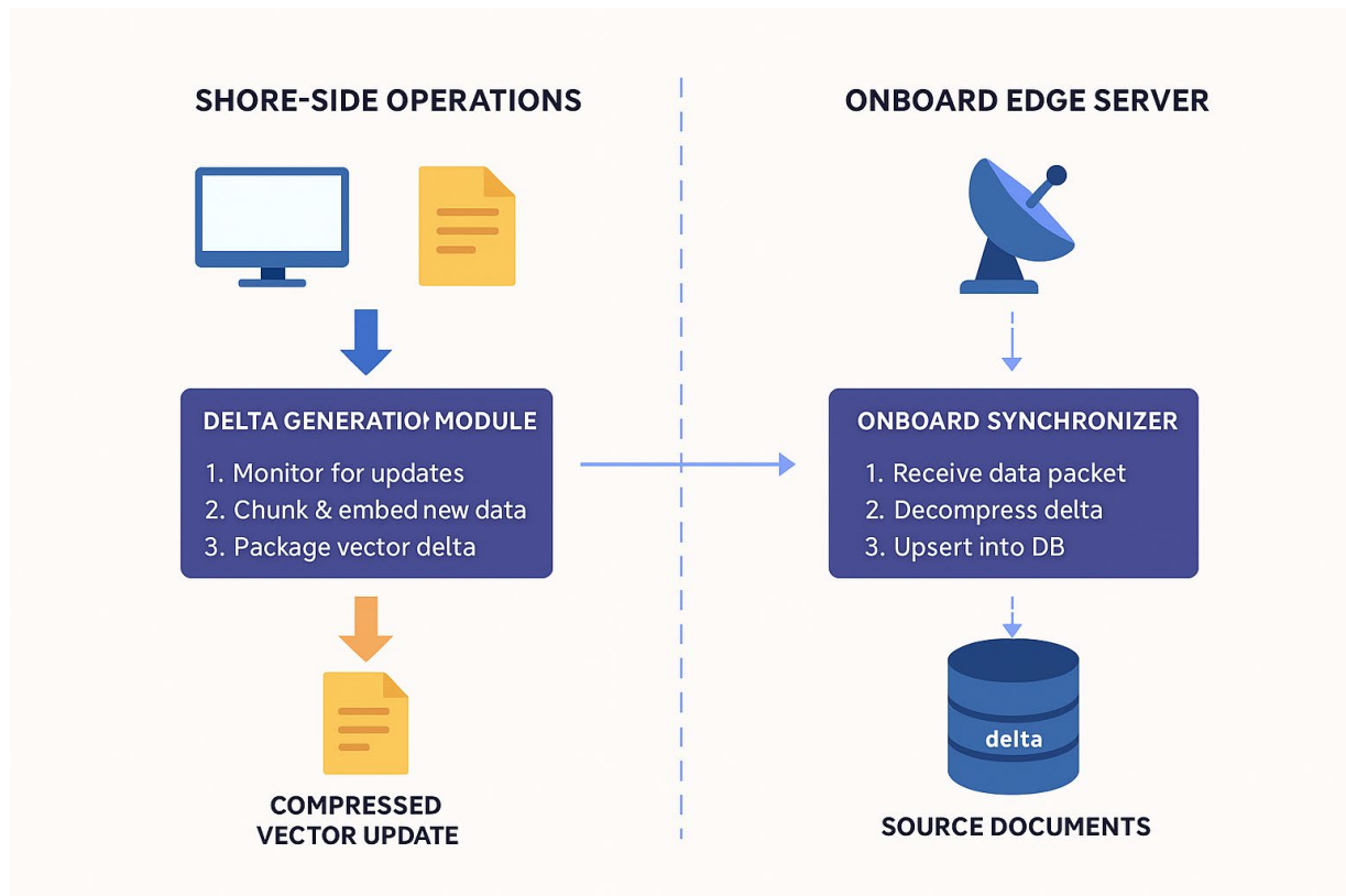
Figure 1: Hybrid Synchronization Mechanism
