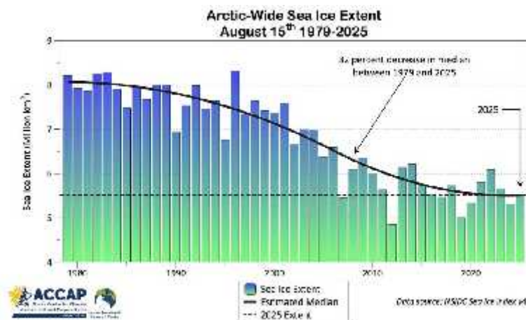
Figure (8): Arctic Sea Ice Extent
