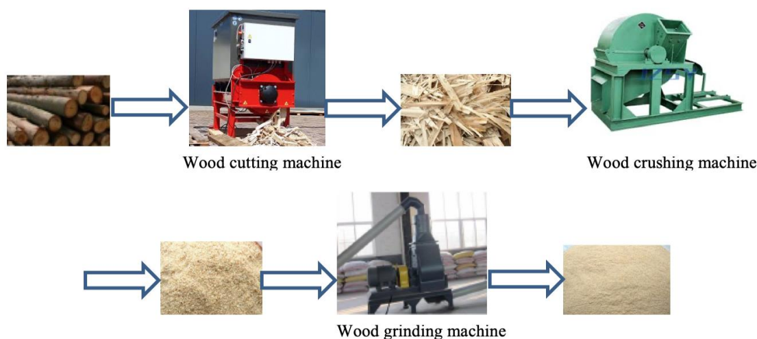
Figure 1: Preparation of wood powder [19].
