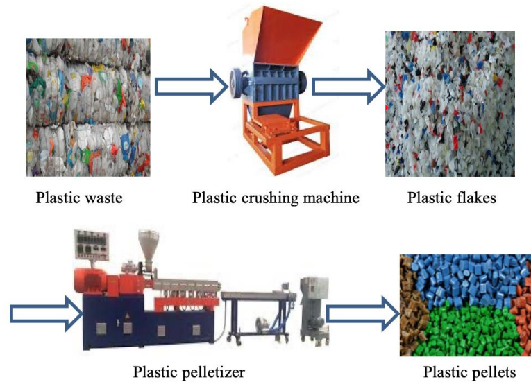
Figure 2: Crushing and pelletizing process.
