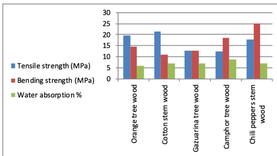
Figure 6: Tensile strength, bending strength, and water absorption for WPC produced from recycled HDPE and different types of agriculture wastes.
