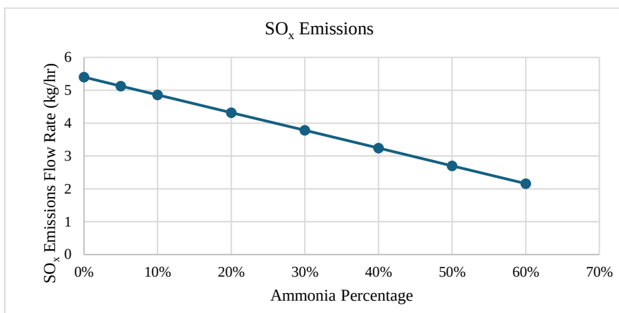
Figure 6: SO x emissions versus ammonia percentage.
