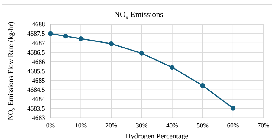
Figure 7: NO x emissions versus hydrogen percentage.
