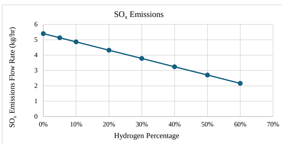
Figure 9: SO x emissions versus hydrogen percentage.
