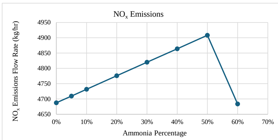
Figure 4: NO x emissions versus ammonia percentage.
