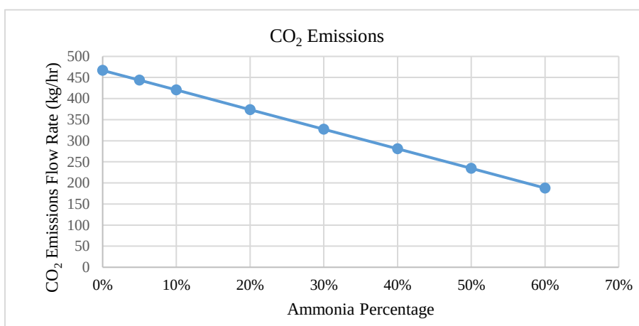
Figure 5: CO 2 emissions versus ammonia percentage.
