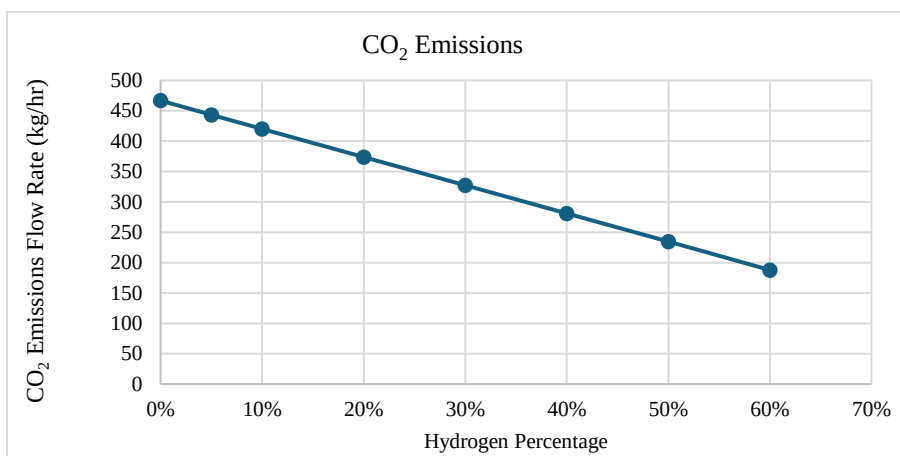
Figure 8: CO 2 emissions versus hydrogen percentage.
