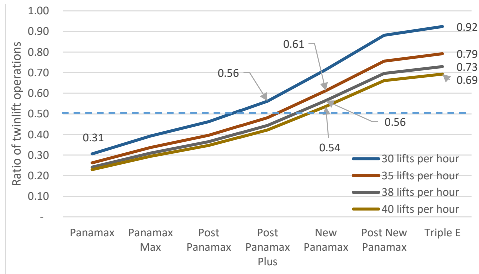
Figure 3: Twinlift Operation Ratios for a Mixed Bay of 20ft and 40ft Containers
